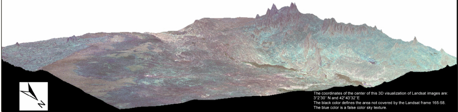
3D visualization of a Landsat composite mosaic of Southern Somalia (closest city is Baydhabo) False colour composite RGB-123, Vertical exaggeration 3x, view from NE
