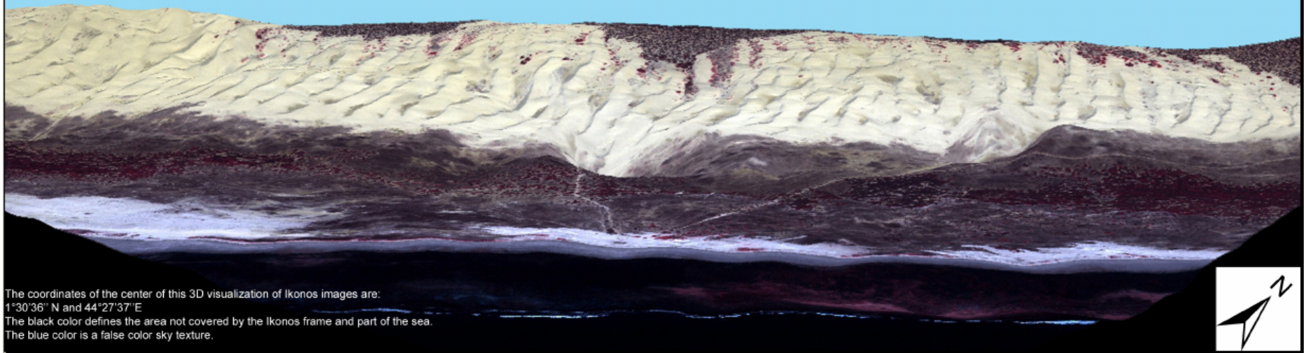
3D Visualization of a Ikonos image of Southern Somalia (closest city Marka) False colour composite RGB-321, Vertical exaggeration 5 x, View from SE
